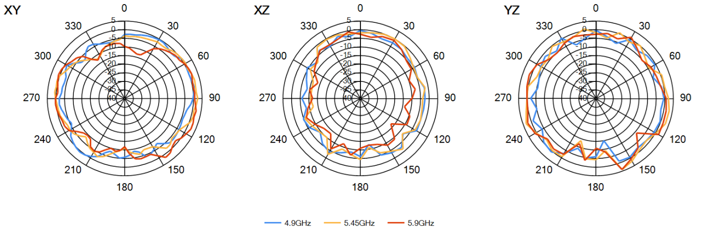
All data measured on SRF2W021-100 in a loaded condition adhered to a plastic carrier in free space
